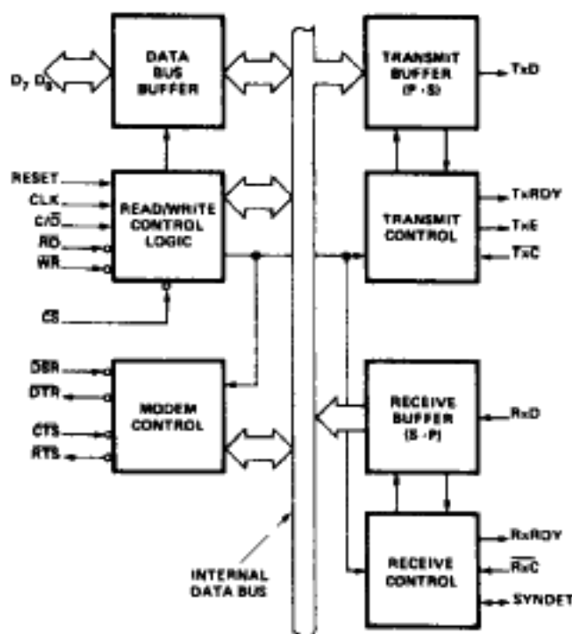
Figure 1. Block Diagram
