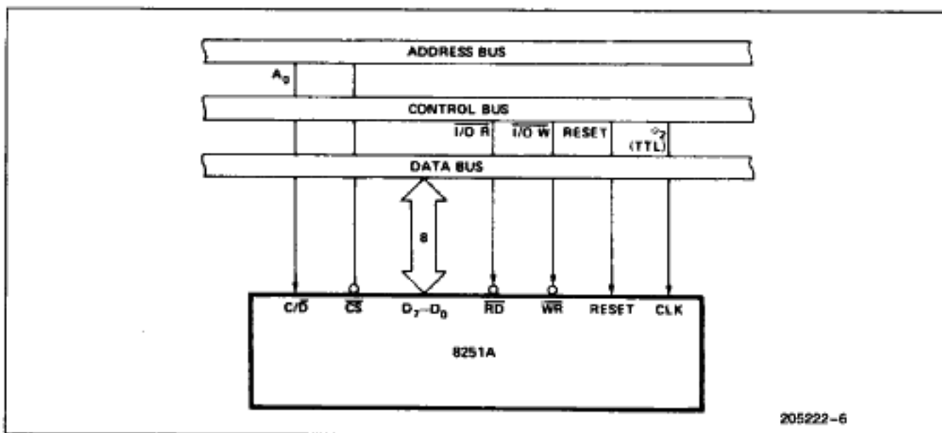
Figure 6. 8251A Interface to 8080 Standard System Bus
